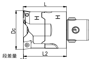
段差切削
