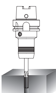
Reaming 铰削
